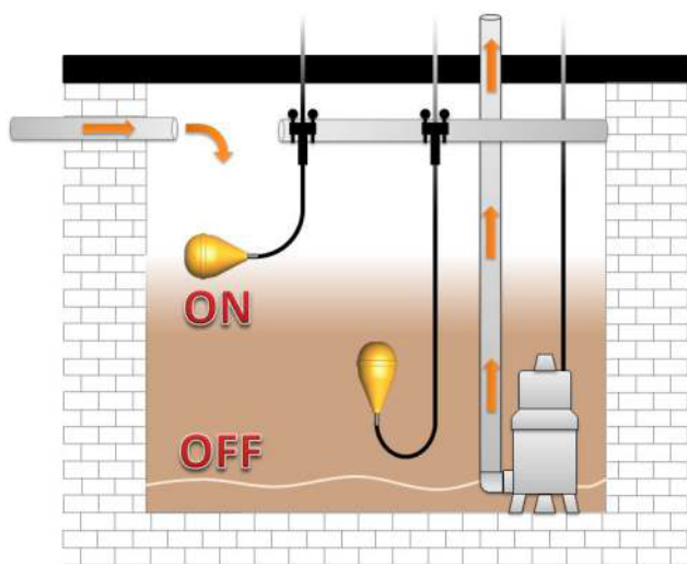
Hight level starts the pump
